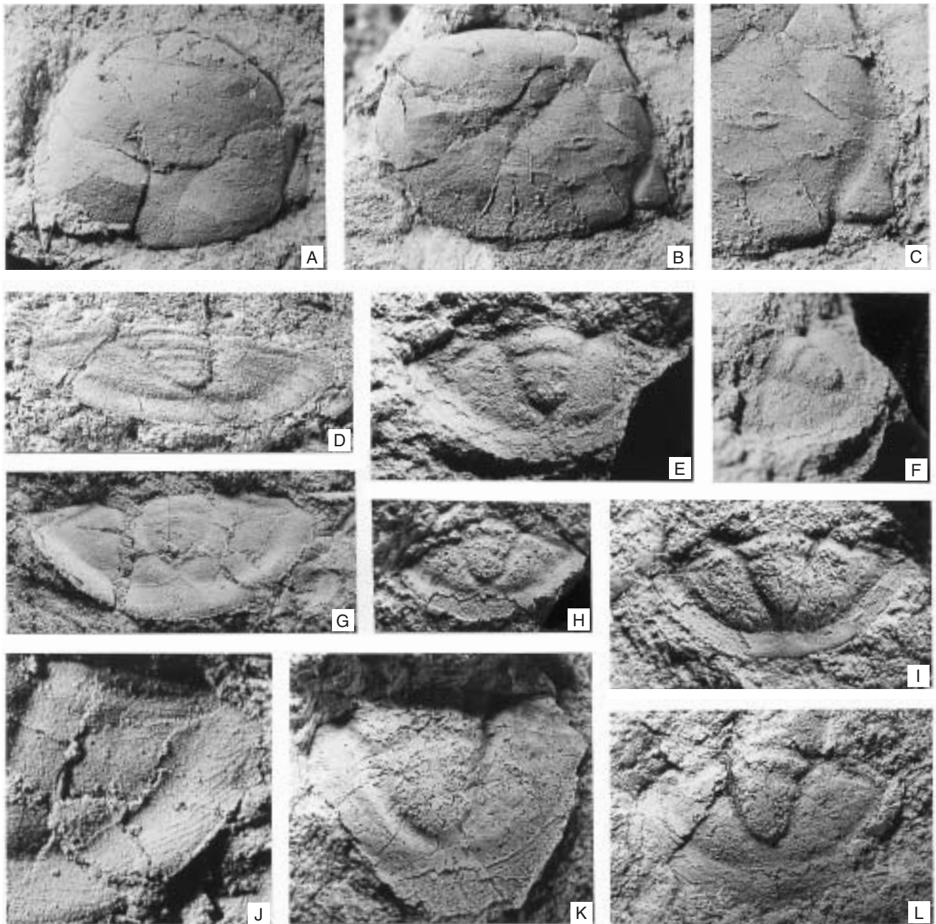
Text-fig. 35. Pricyclopyge oceanitis sp. n.
