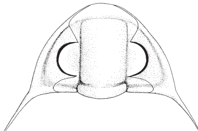
Text-fig. 15. Agerina clymene sp. n. Reconstruction of the cephalon. Approximately ×10.
