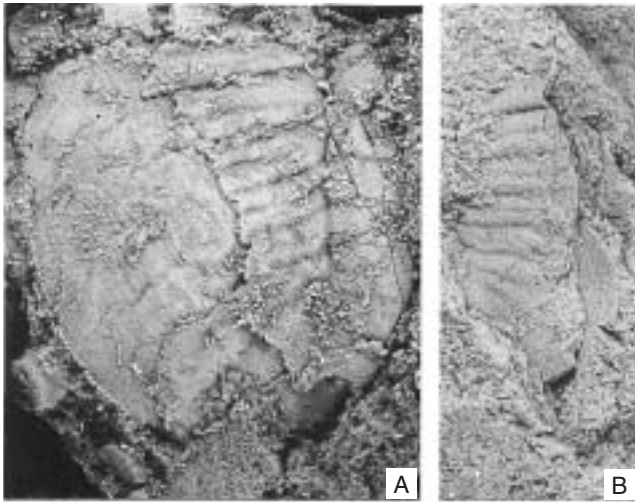
Text-fig. 25. Niobina sp. A – incomplete pygidium, latex cast of exterior, MM 129, ×2.5; B – fragment of pygidium, internal mould, PCZCU 1581, ×2.5. Mílina Formation, Olešná.
