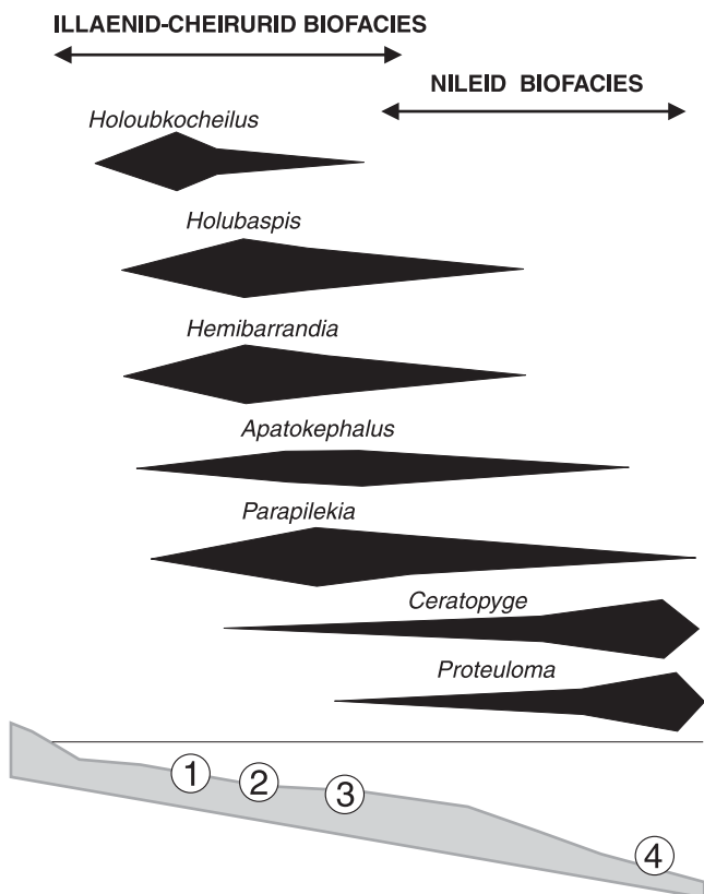
Text-fig. 7. Reconstruction of depth-related distribution of index trilobite genera in the Milina Formation. Number indicate approximate depth-related position of trilobite-bearing localities (1 – Holoubkov, 2 – Kvaň, 3 – Olešná, 4 – Úvaly).
