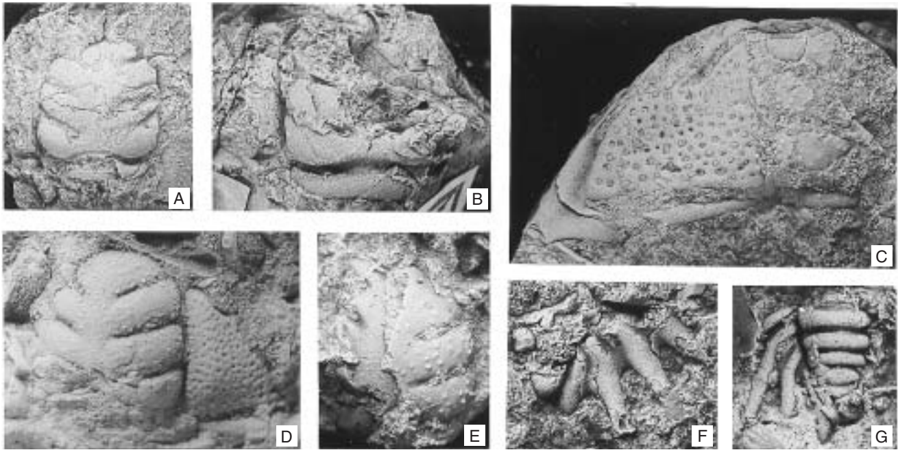
Text-fig. 18. Parapilekia ferrigena MERGL, 1994.
