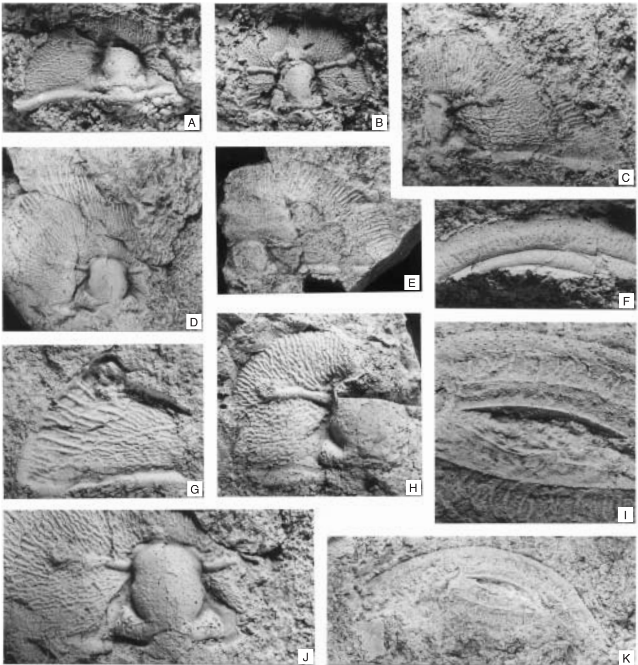
Text-fig. 40. Harpides grimmi BARRANDE, 1852.
