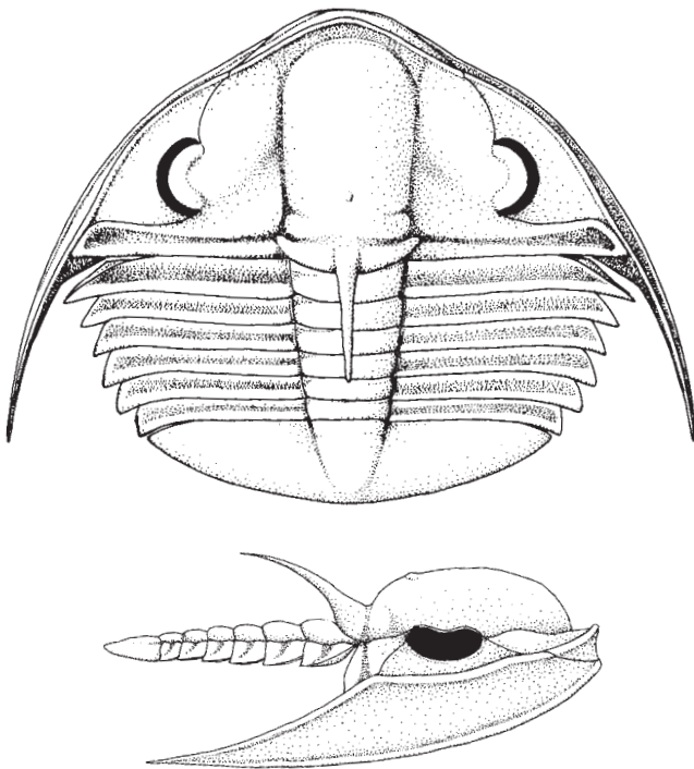
Text-fig. 39. Celdometopus kloučeki (VANĚK, 1965). Reconstruction and lateral view to the exoskeleton. Approximately \times 10 .
