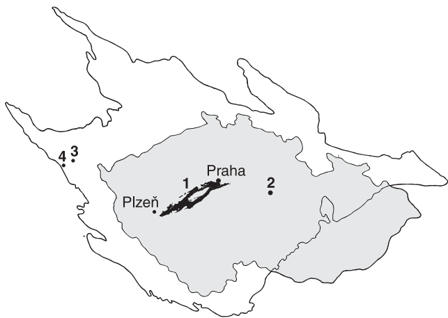
Text-fig. 1. The Bohemian Massif with the Ordovician of the Barrandian area (1) and the trilobite-bearing localities in Železné hory area in East Bohemia (2), Hof (Leimitz Shales) (3) and Vogtendorf (Vogtendorf Formation) (4) in Bavaria.
