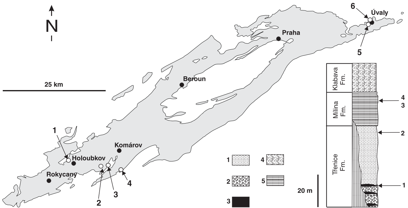
Text-fig. 2. The Ordovician of the Prague Basin (A) with trilobite-bearing localities (1 – Holoubkov, 2 – Cheznovice, 3 – Olešná, 4 – Kvaň, 5 – Úvaly, Škvorec enclosure, 6 – Úvaly, Vinice) and general lithostratigraphy of the Tremadocian of the Prague Basin (1 – greywacke, 2 – conglomerate, 3 – haematite, 4 – siltstone, 5 – chert).
