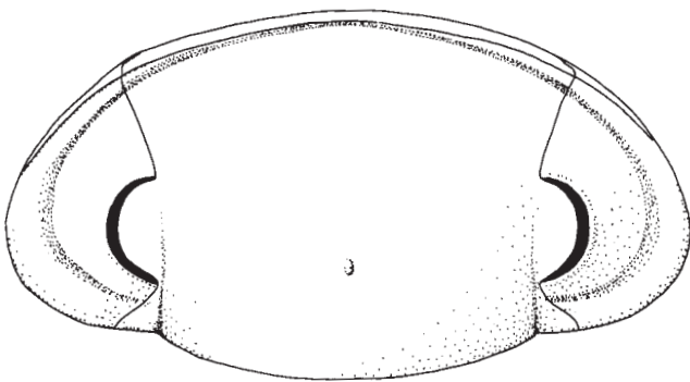
Text-fig. 10. Ottenbyaspis broeggeri (RŮŽIČKA, 1926). Reconstruction of the cephalon. Approximately \times 6 .
