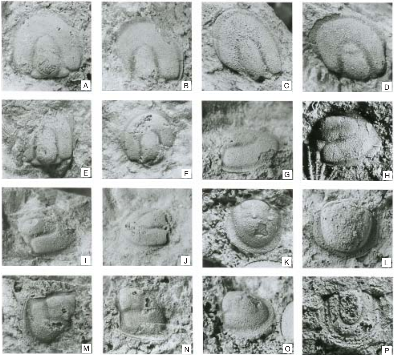
Text-fig. 8. Geragnostus peki (MERGL, 1984)
