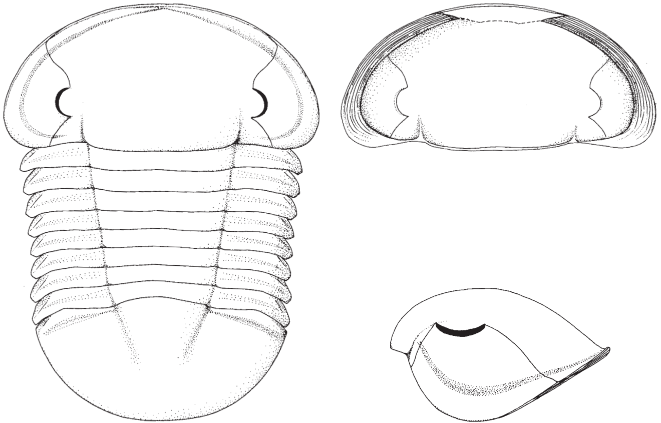
Text-fig. 13. Hemibarrandia klouceki sp. n. Reconstruction of the exoskeleton, ventral side of the cephalon and lateral view to the cephalon. Approximately \times 1.5 .
