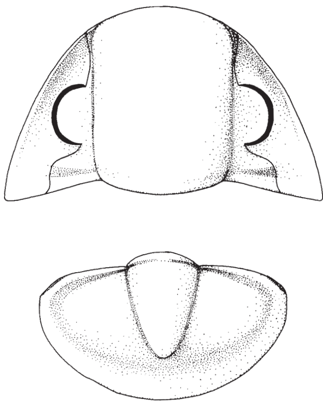
Text-fig. 37. Platypeltoides perseis sp. n. Reconstruction of the cephalon and the pygidium. Approximately \times 2 .
