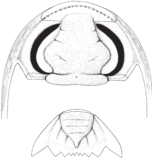
Text-fig. 34. Apatokephalus dagmarae MERGL, 1984. Reconstruction of the cephalon and the pygidium. Approximately \times 6 .
