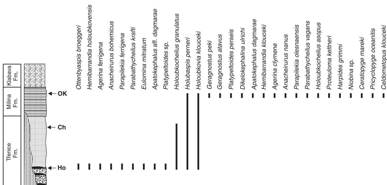
Text-fig. 6. Stratigraphical column of the Třenice and Mílina Formations in the southwestern part of the Prague Basin and distribution of trilobites. Localities: Ch – Cheznovice, Ho – Holoubkov, OK – Olešná and Kván.
