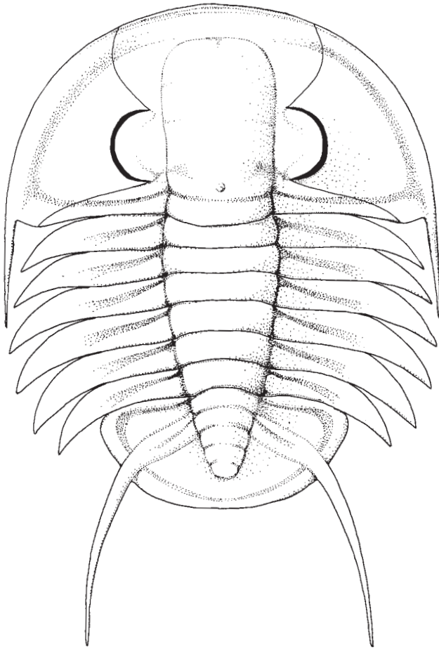
Text-fig. 27. Ceratopyge mareki MERGL, 1984. Reconstruction of the exoskeleton. Approximately \times 4 .
