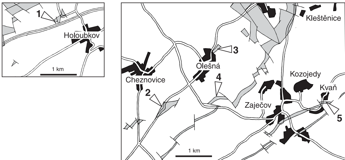
Text-fig. 4. Outcropping Tremadocian rocks in the Holoubkov area (A) and the Komárov area (B) with discussed trilobite-bearing localities (1 – Holoubkov, 2 – Cheznovice, 3 – Olešná, 4 – Mílina, 5 – Kvaň).
